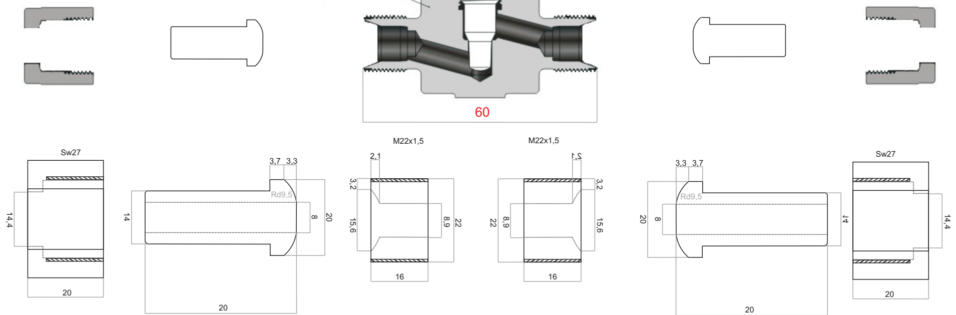
Union nut M22x1,5 Welding nipple Connection end M22x1,5 Connection end M22x1,5 Welding nipple Union nut M22x1,5
